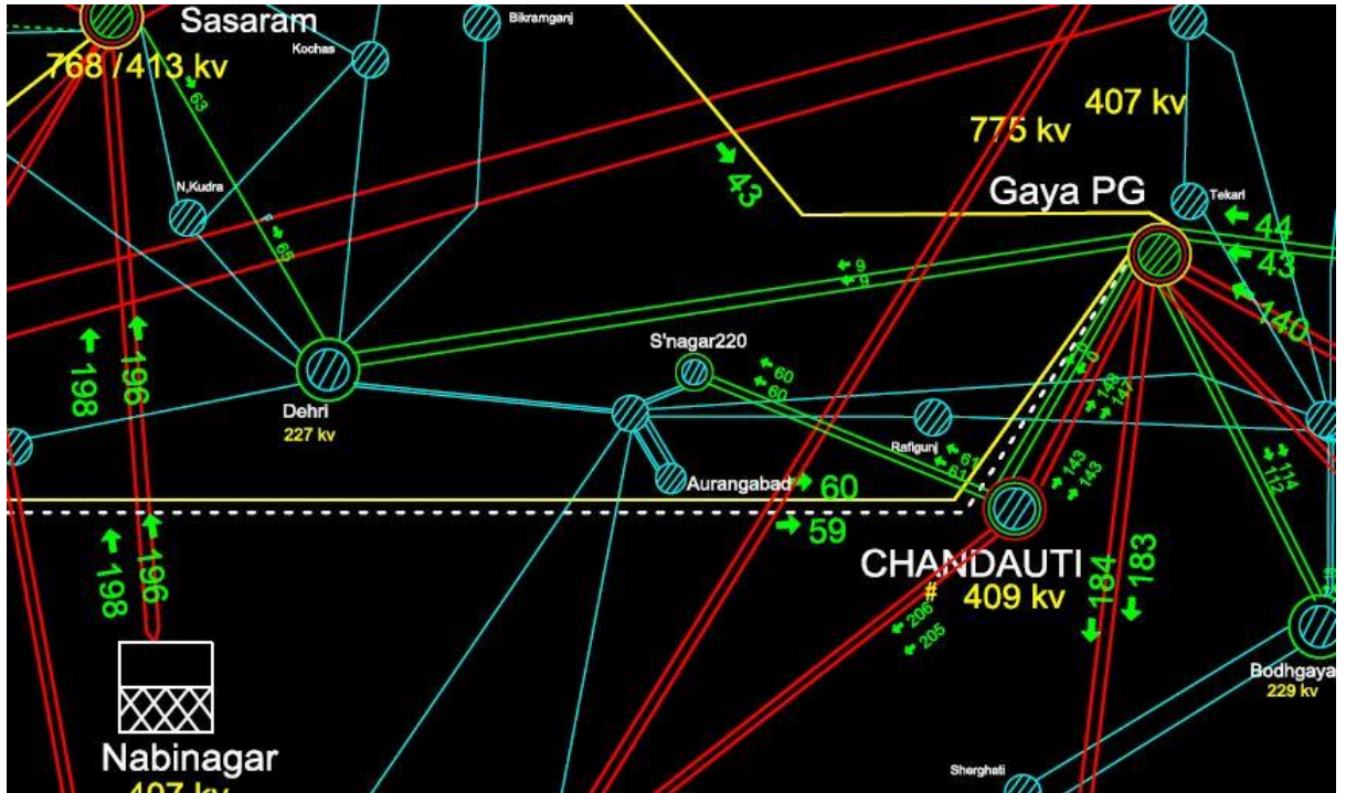
Figure 2: SCADA snapshot for of the system
