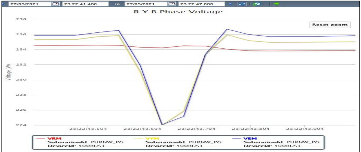
Figure 3: Three phase voltage captured by New Purnea PMU shows existence of fault in Y and B phase at 23:22 hrs. Around 10 kV dip has been observed in Y and B phase voltage at New Purnea PMU. Fault clearing time was around 100 ms.
