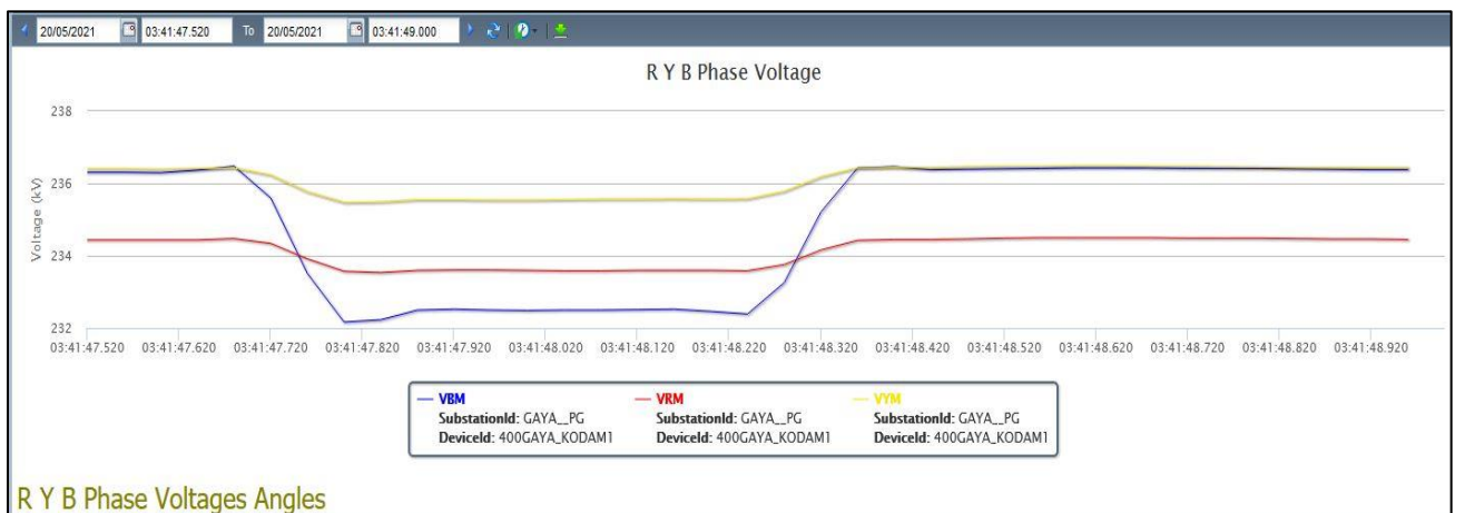
Figure 3: Three phase voltage captured by Gaya PMU shows existence of B phase to earth fault at 03:41 hrs. Around 4 kV dip has been observed in B phase voltage at Gaya PMU. Fault clearing time was around 500 ms.
