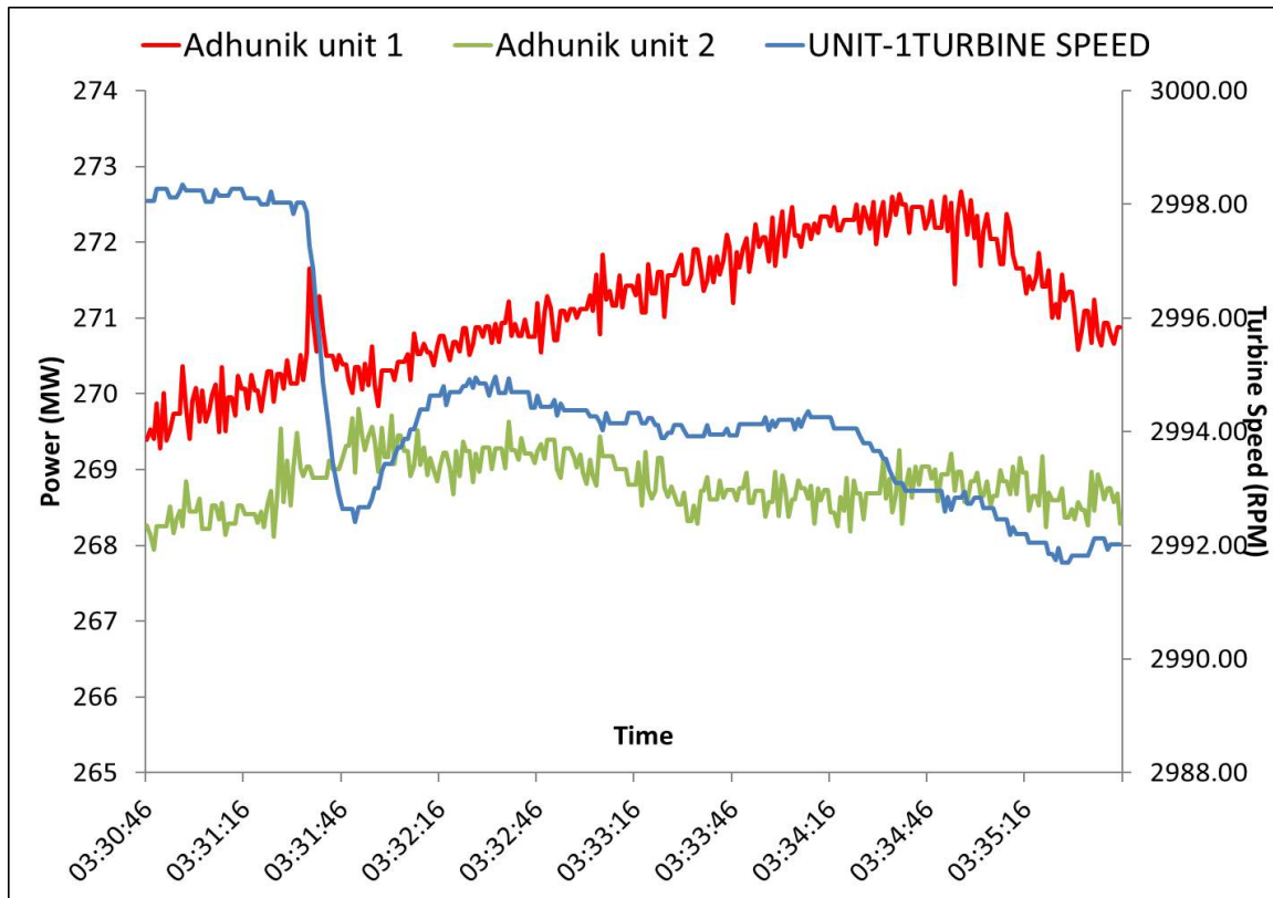
Annexure 1: Variation of generation of regional generating units during frequency change (plotted based on data shared by generating station)
