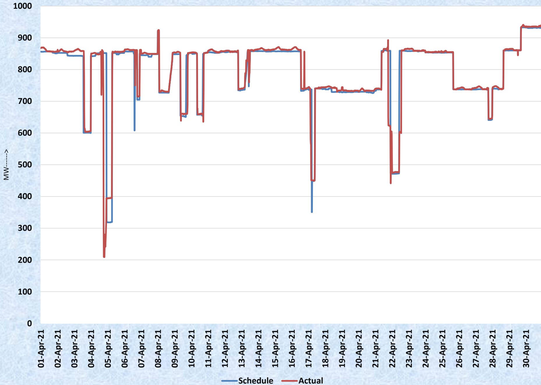
Schedule vs Actual Drawl of Bangladesh From 1st April to 30th April
