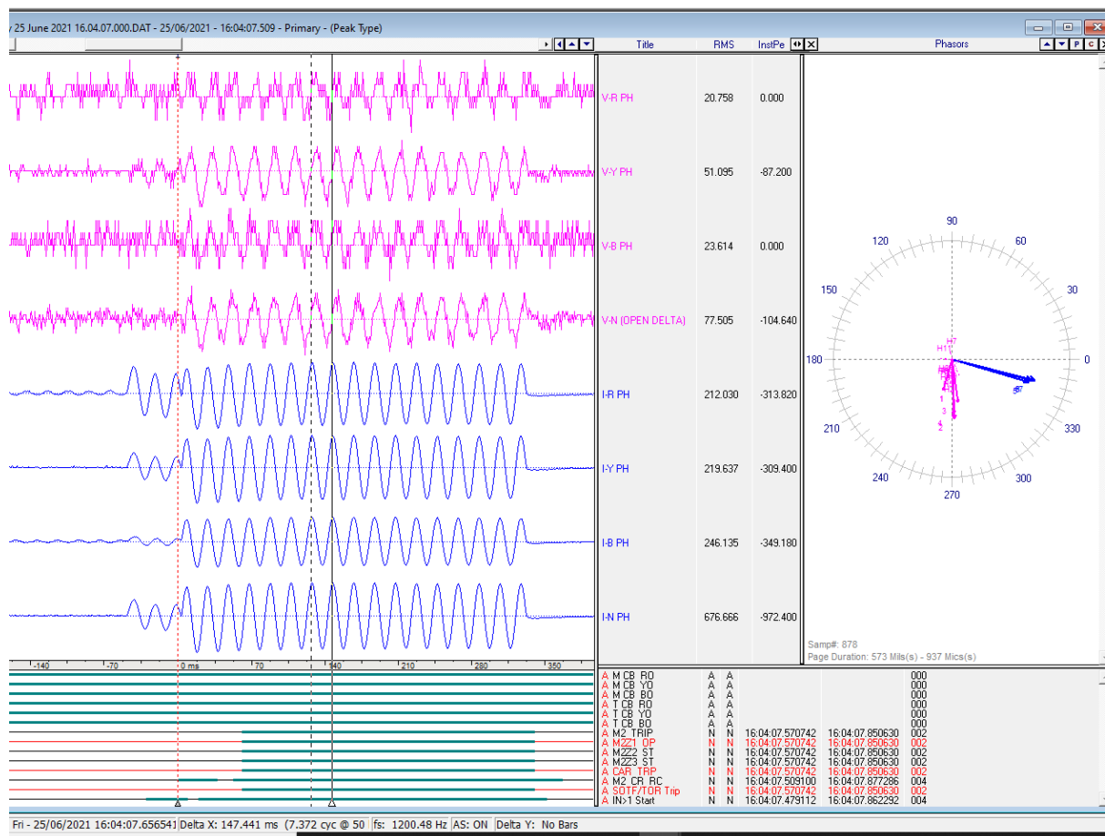
DR record of Sonenagar Ckt-1 at the time of event
