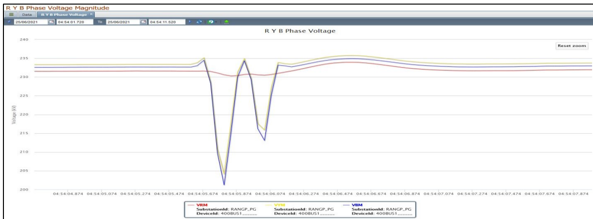
Figure 3: Three phase voltage captured by Rangpo PMU shows existence of Y-B fault at 04:54 hrs. Around 30 kV dip has been observed in Y phase and 35 kV dip is observed in B phase voltage at Rangpo PMU. Two consecutive dips in Y-B phase are captured. Fault clearing time was around 240 ms.
