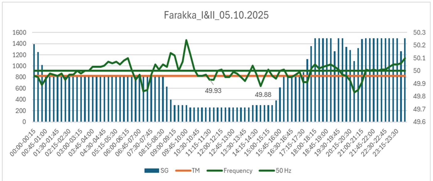
SG less than Technical Minimum, despite eligible for SCED Technical Minimum.
